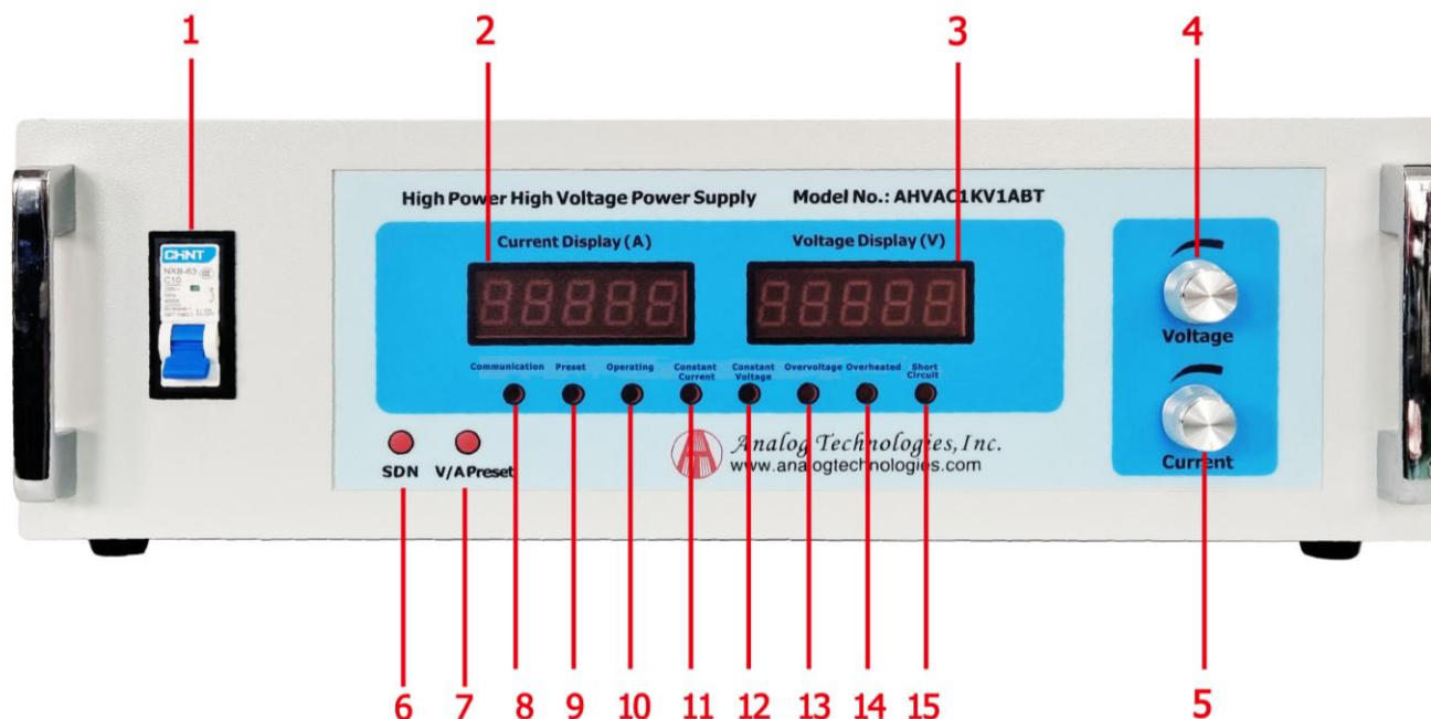
Figure 2. Front Panel
