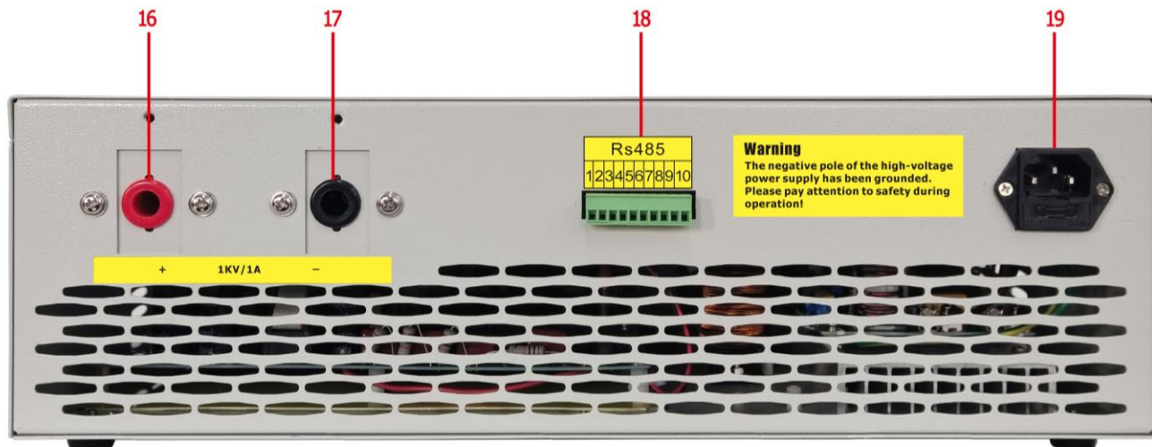
Figure 3. Back Panel
