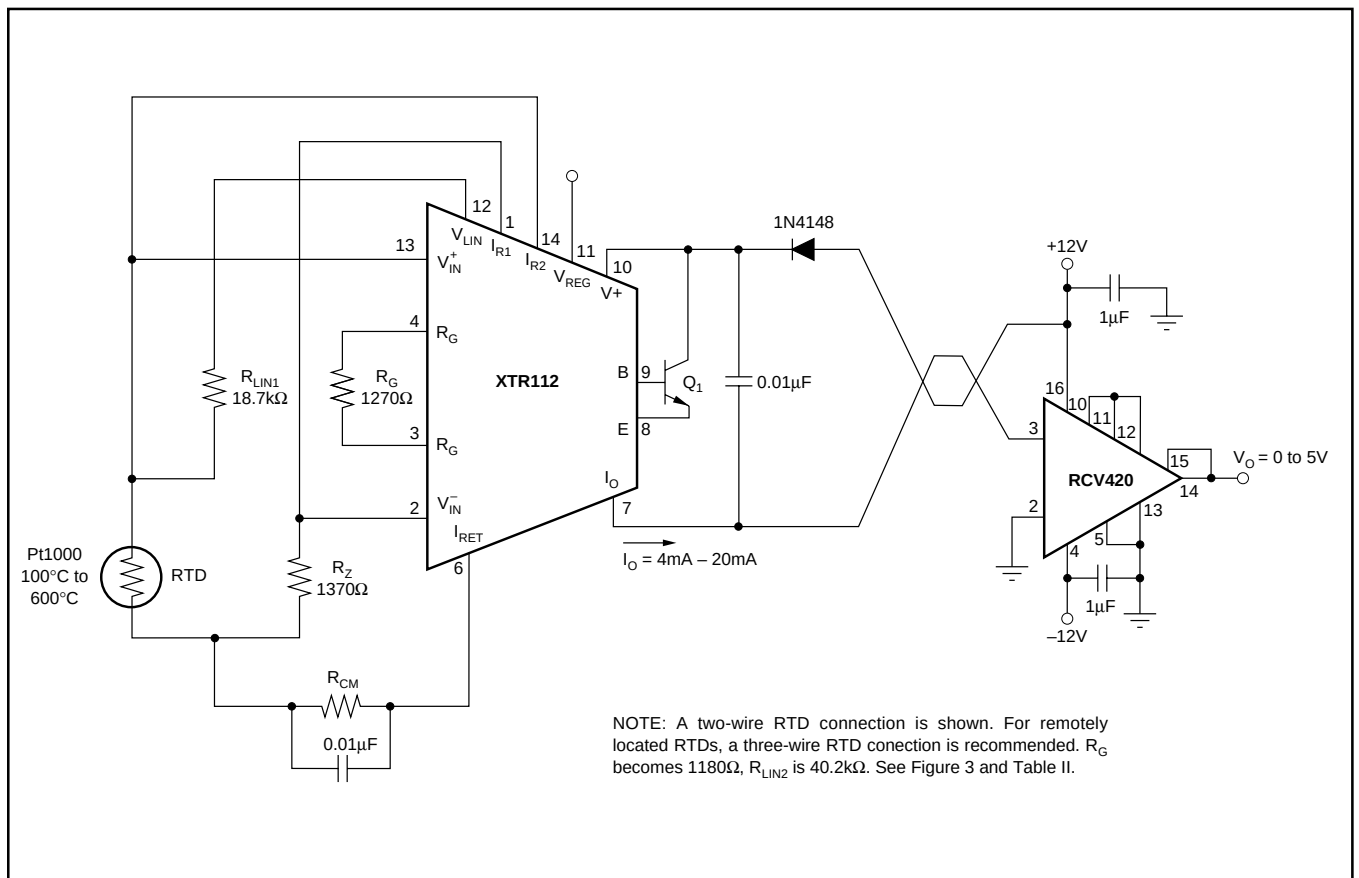
FIGURE 7. \pm 12\text{V} Powered Transmitter/Receiver Loop.
